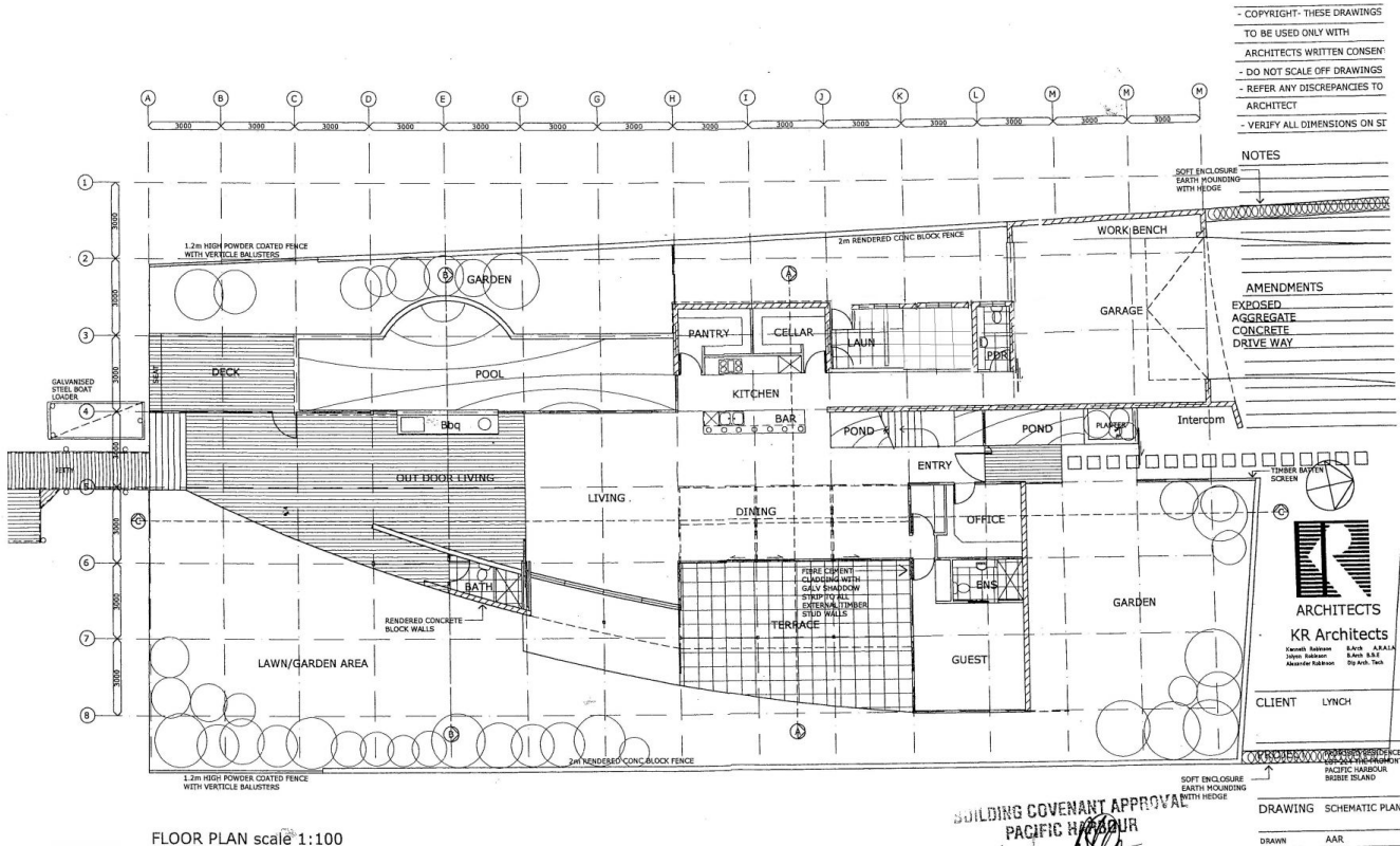
FLOOR PLAN scale 1:100
