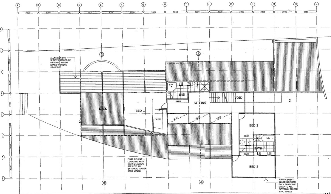
LEVEL 1 PLAN scale 1:100
